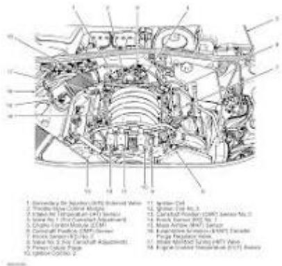
Figure Q&A: Audi A6 Avant 2.8 - Engine Diagram, P1196, P0411 &
